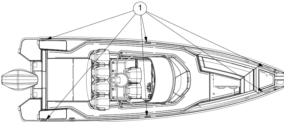
(1) Fastening points
